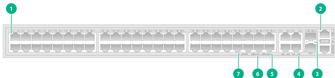
图2-2 R3900-S51-G-DP 指示灯
